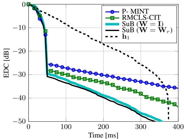
Fig. 2: EDC of the true RIR \mathbf{h}_1 and EDC of the EIR obtained using regularized P-MINT, regularized RMCLS-CIT, regularized SuB with \mathbf{W} = \mathbf{I} , and regularized SuB with \mathbf{W} = \mathbf{W}_r ( E_m = -33 dB, L_w = 50 ms)
